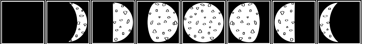
New Moon
