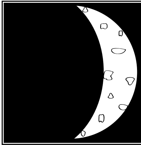
Waxing Crescent
