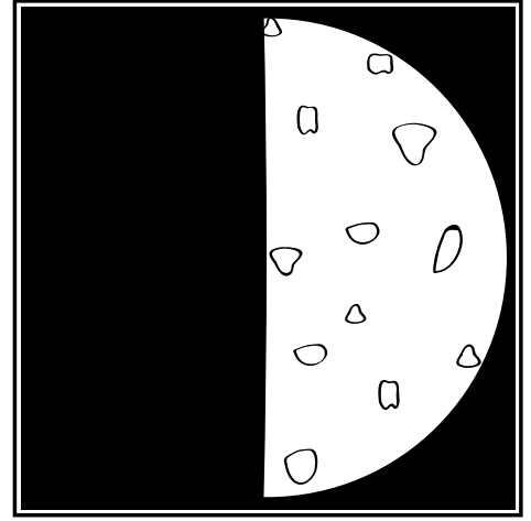
First Quarter
