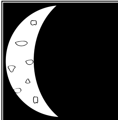
Waning Crescent
